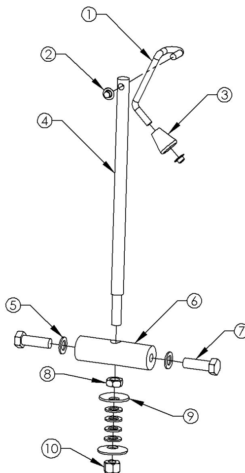
Fig. 6 HEIGHT ADJUSTMENT
