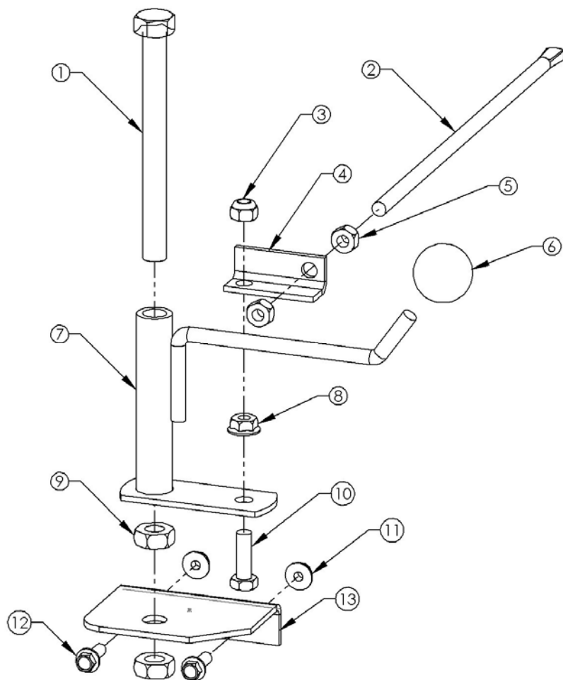
Fig. 5 STANDARD ENGAGE
